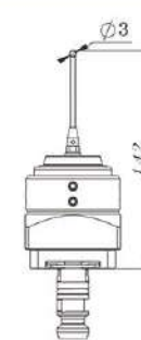
RHS centering sensor 3mm tip spring loaded
