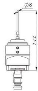
RHS Macro compatible probe spring loaded 8mm tip dia
