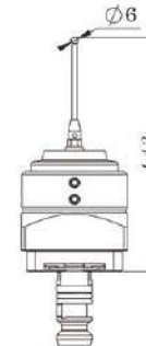
System 3R 3R-656.31-3P Measuring probe Ø6 mm Macro
