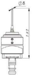
RHS Macro compatible probe spring loaded 5mm tip dia
