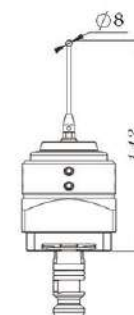
System 3R 3R-656.31-3P Measuring probe Ø8 mm Macro
