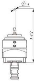
RHS Macro compatible probe spring loaded 4mm tip dia
