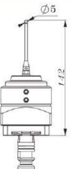
System 3R 3R-656.31-3P Measuring probe Ø5 mm Macro
