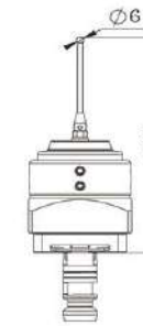
RHS Macro compatible probe spring loaded 6mm tip dia
